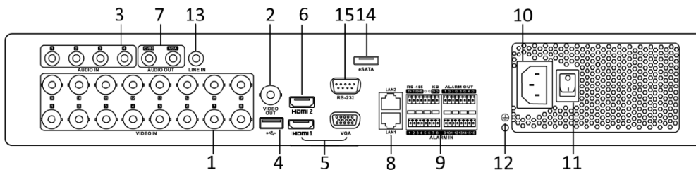
Figure 1-11 Rear Panel
