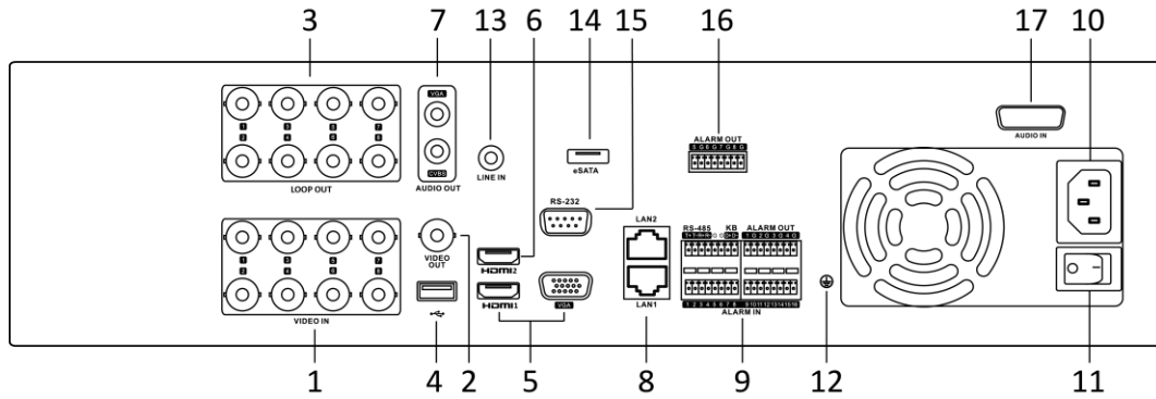
Figure 1-12 Rear Panel
